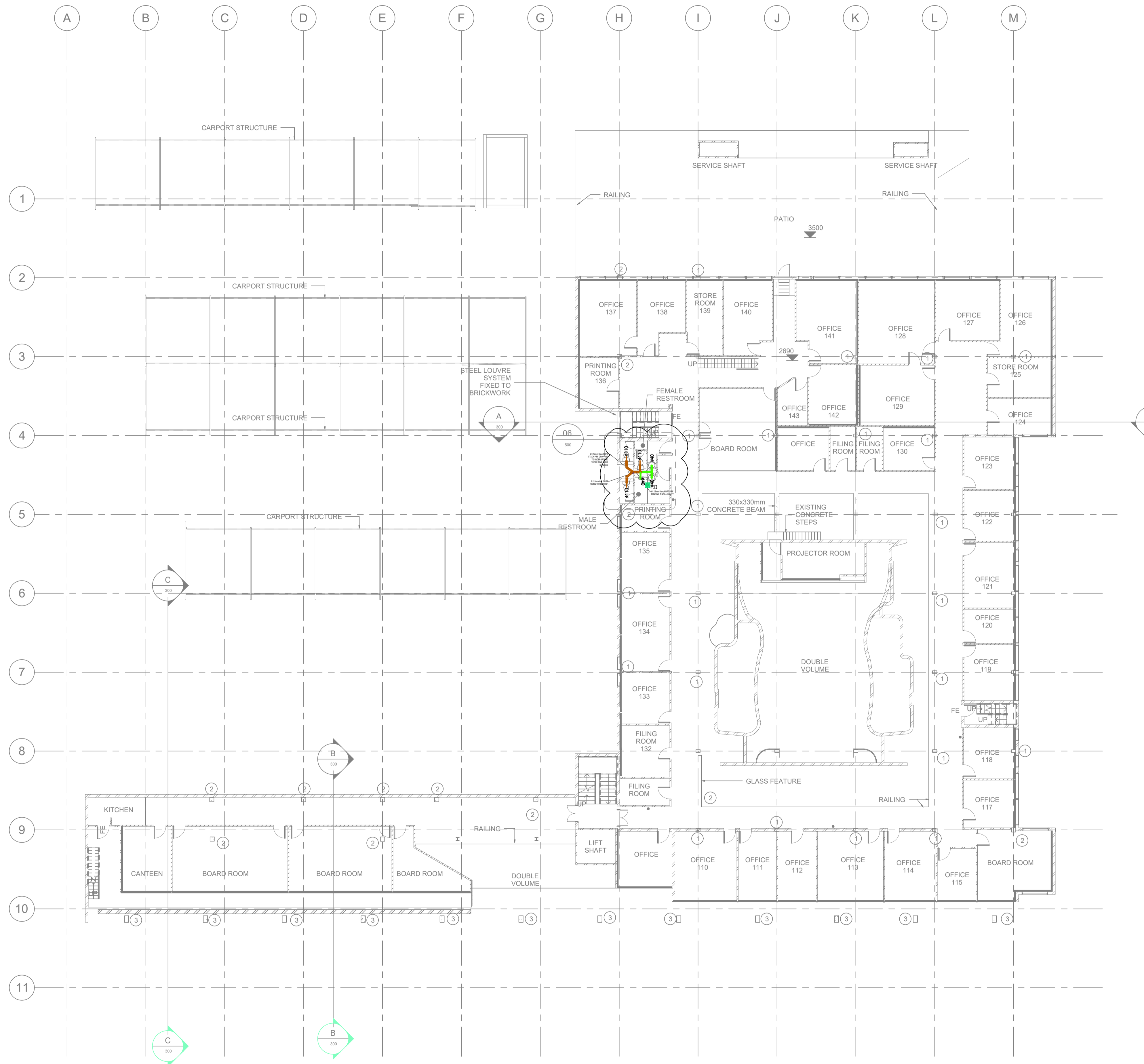
FIRST FLOOR INTERNAL DRAINAGE LAYOUT 1 : 150
